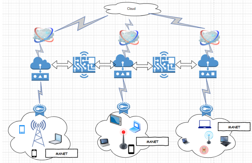
Figure 2: Cloud-MANET-IoT framework
